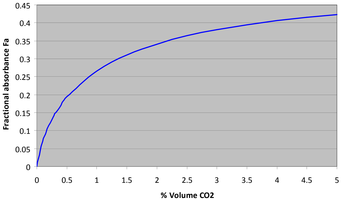
Typical response 0-5% volume CO2
