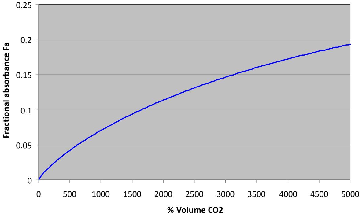
Typical response 0-5000 ppm CO2
